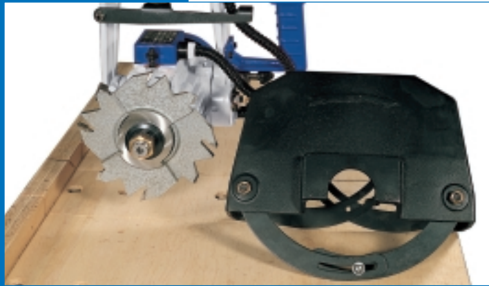
Dado Head Guard 720150130000 (12" x 2-3/8") 720150140000 (12" x 3-15/16")
